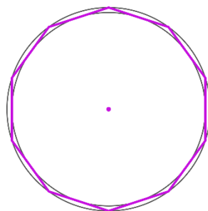
Decagon 10 Sided Circular Approximation
