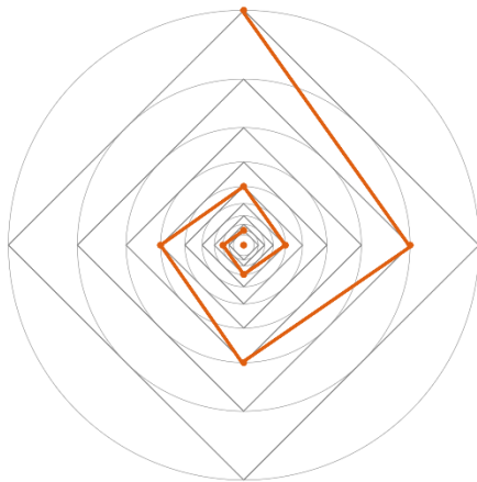
Connecting Points Quadragonal Convergence
