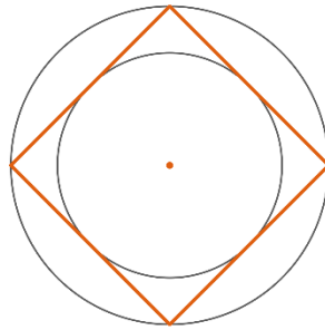
Quadragon 4 Sided Circular Approximation
