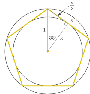
3. Pentagon Convergence Factor
