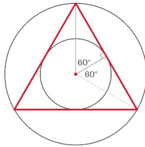
2. Triagon Radii Angle Relationship
