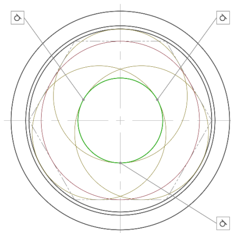
STEP 6 FLAME CONSTRUCTION GEOMETRY 2
