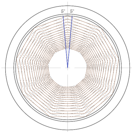
STEP 17 WEB CONSTRUCTION GEOMETRY 2
