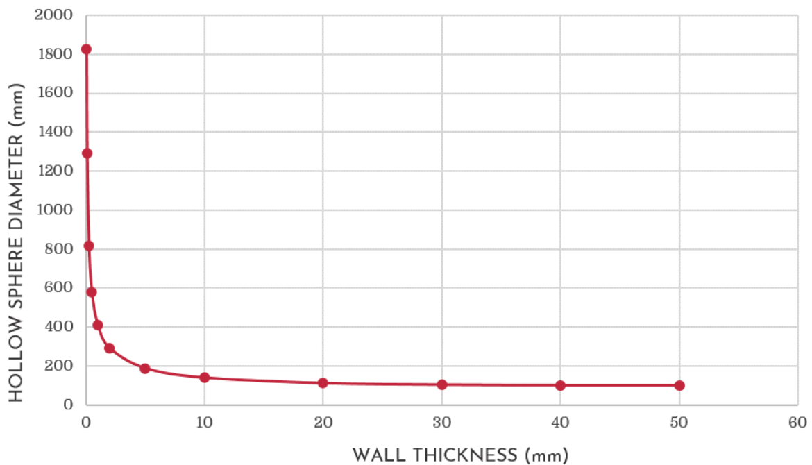
HOLLOWING SPHERE GROWTH (Ø100 mm)
