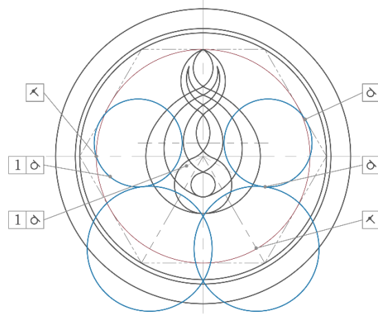
STEP 11 RECEPTACLE CONSTRUCTION GEOMETRY 1
