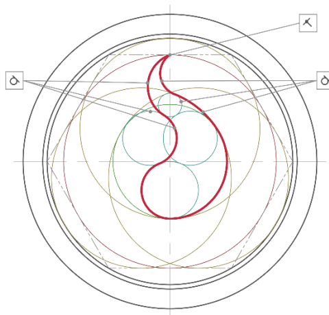
STEP 8 FLAME CONSTRUCTION
