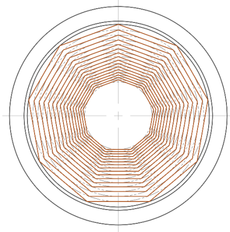
STEP 16 WEB CONSTRUCTION GEOMETRY 1
