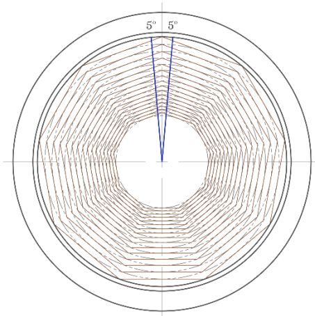
STEP 17 WEB CONSTRUCTION GEOMETRY 2
