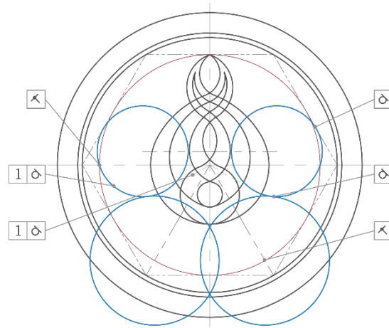
STEP 11 RECEPTACLE CONSTRUCTION GEOMETRY 1
