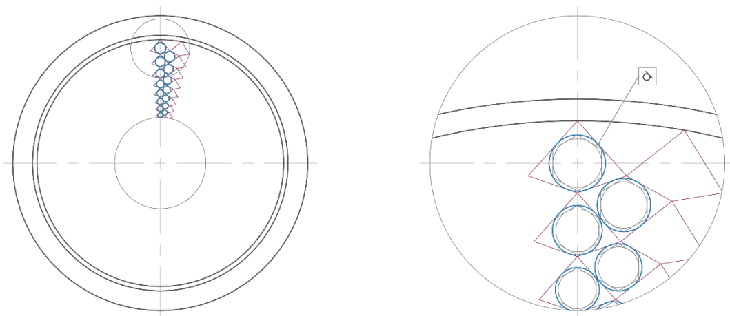
STEP 19 WEB CONSTRUCTION GEOMETRY 4
